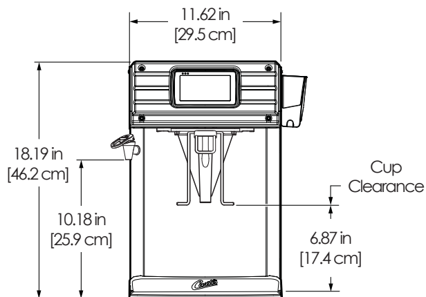
Front View - CGC1
