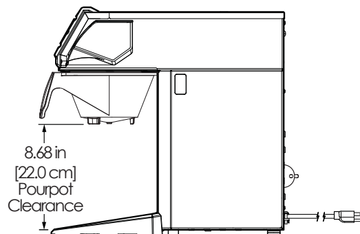
Side View - CGC1 with Large Brew Basket
