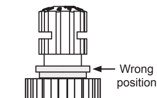
Locking collar in wrong position Knob turns but has no effect on foam level
